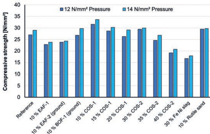
Figure 7: Compressive strength of the calcium silicate masonry units depending on type and share of the industrial aggregates and the pressure
