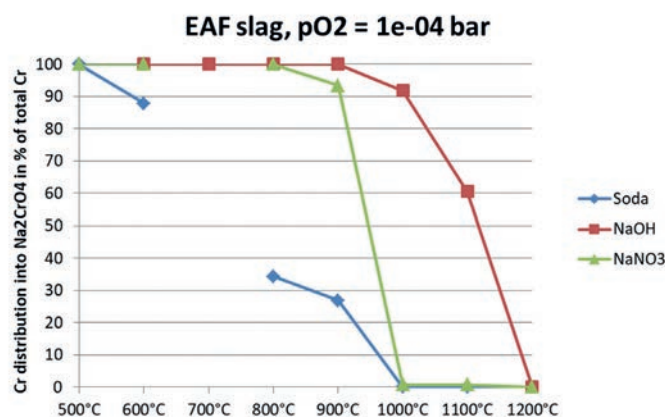
Figure 2: Chromium distribution into the leachable phase Na_2CrO_4 for EAF slag at various roasting temperatures with various additives at p_{O_2} = 1e^{-04} bar
