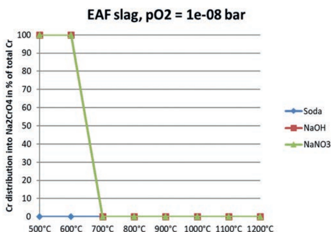
Figure 3: Chromium distribution into the leachable phase Na_2CrO_4 for EAF slag at various roasting temperatures with various additives at p_{O_2} = 1e^{-08} bar
