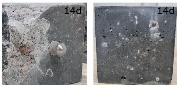
Figure 3: Damage intensities as a function of sample geometry (prism / cube) (w/c = 0.60; free lime = 1.9 wt.%; test temperature = 60°C)
